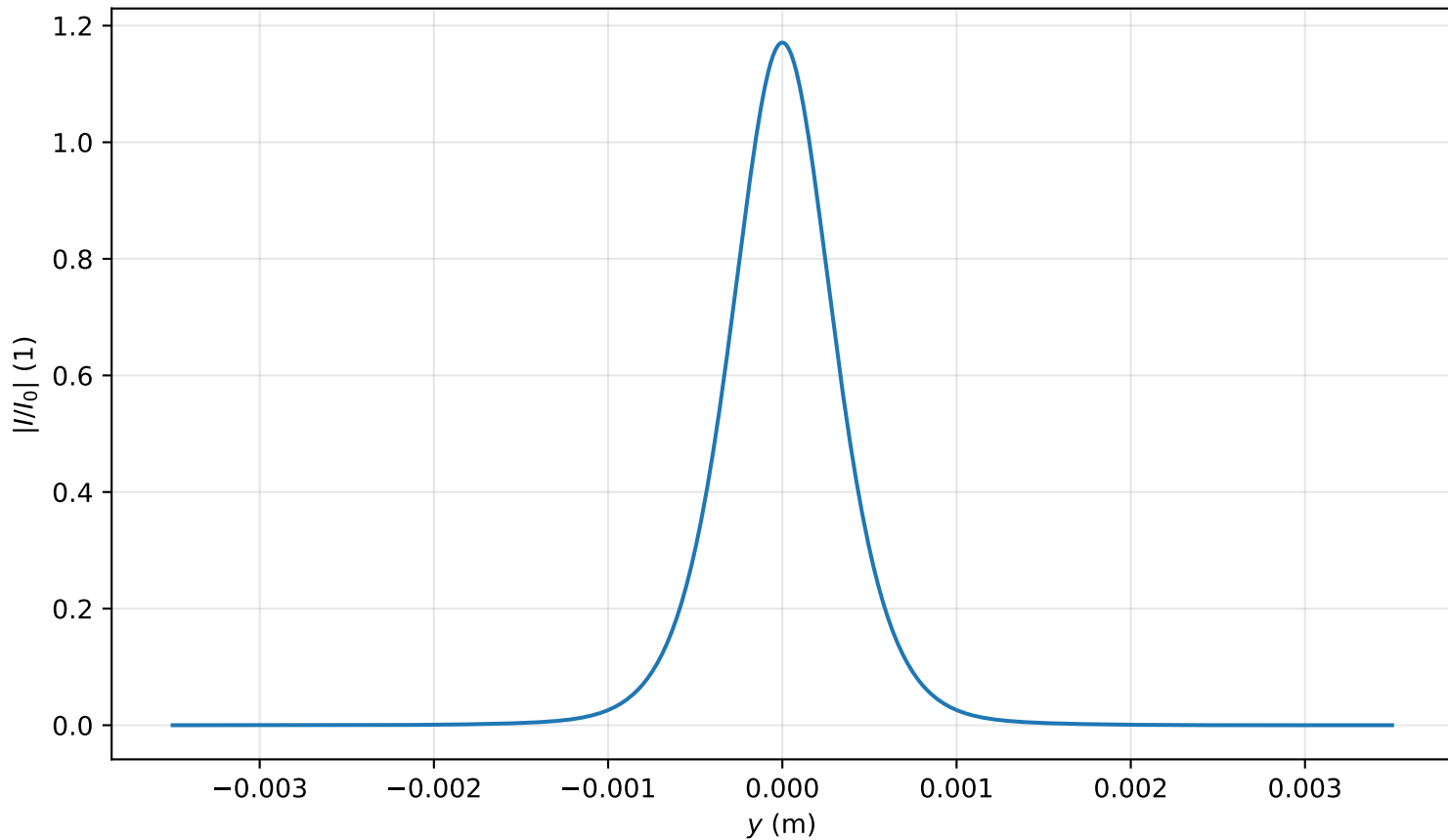
Intensity profile I(x=0, y, z=2.707)/I_0 , P_{in}=0.8P_{cr} , artificial time
